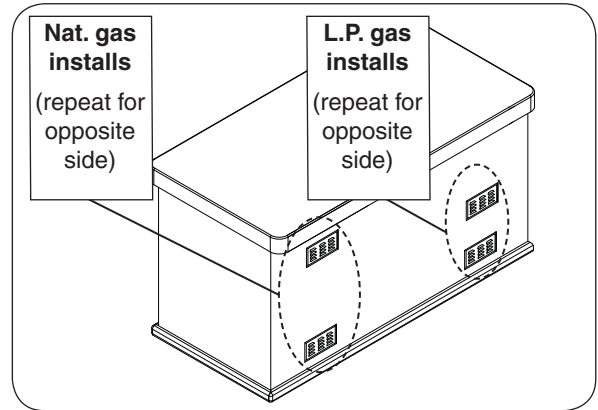
Fig. 8-1 Ventilation detail
