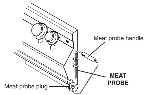
Fig. 24-1 Meat probe detail
