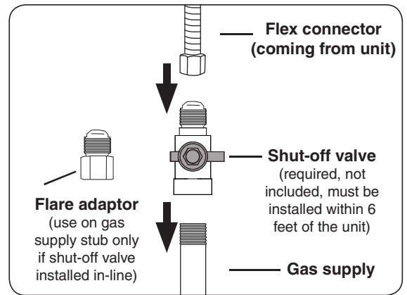
Fig. 19-1 Connecting to a gas line
