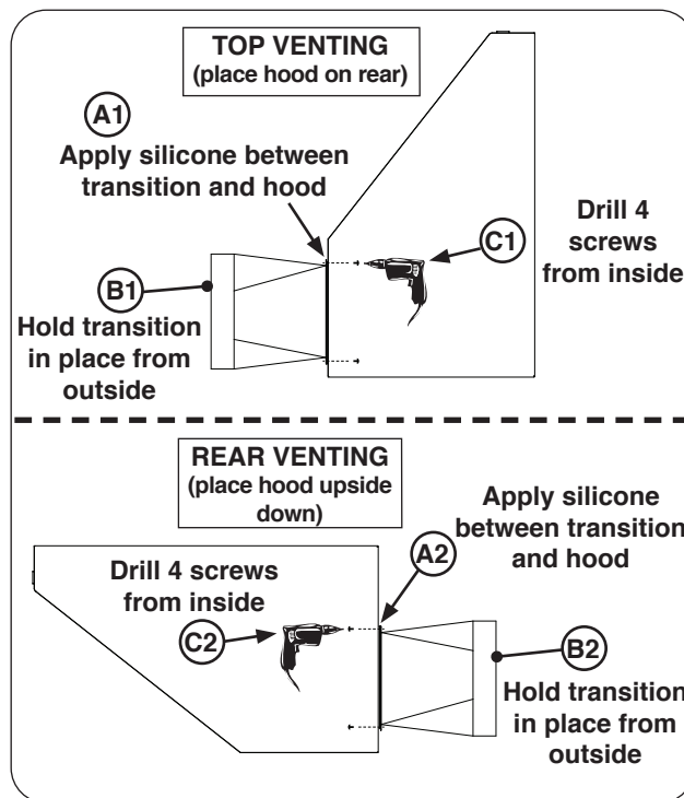
Fig. 14-2 Install transition
