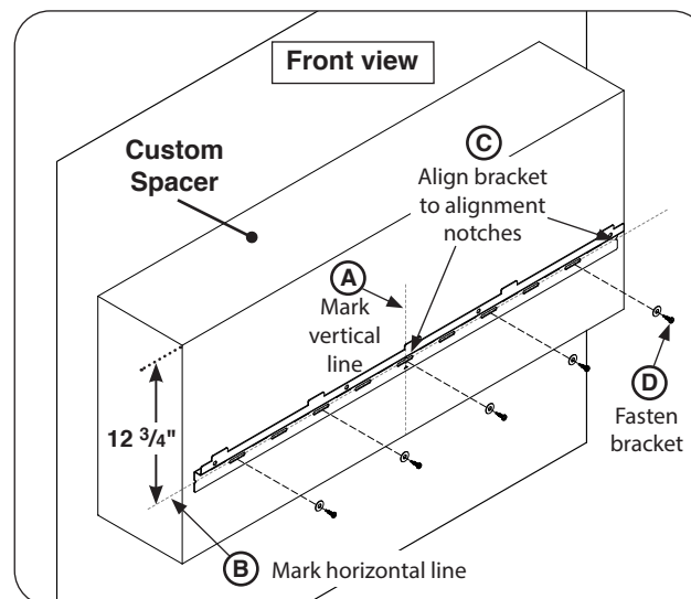
Fig. 14-3 Install bracket to custom spacer
