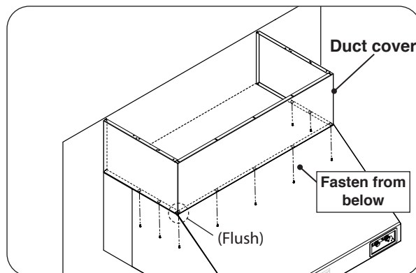
Fig. 19-1 Install Fire Magic Duct Cover
